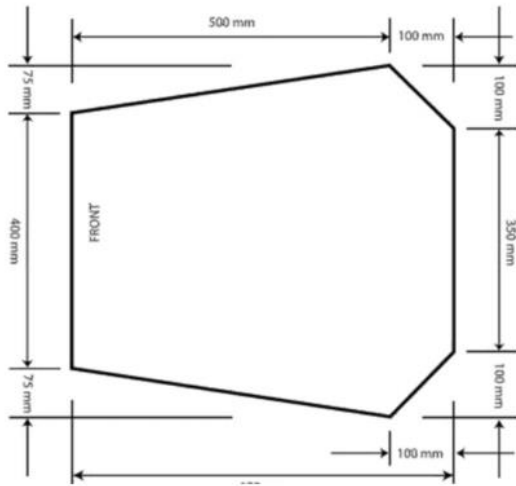
Cockpit opening template of FSAE Rules 2020
